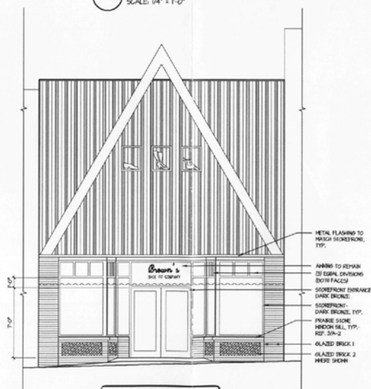
PROPOSED EAST ELEVATION SCALE: 1/4" = 1'-0"
