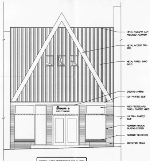
EXISTING EAST ELEVATION SCALE: 1/4" = 1'-0"
