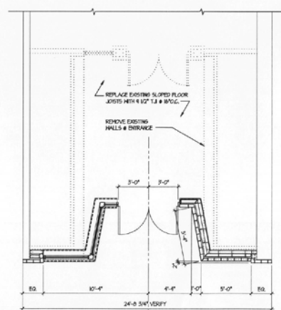
PROPOSED ENTRY PLAN SCALE: 1/4" = 1'-0"
