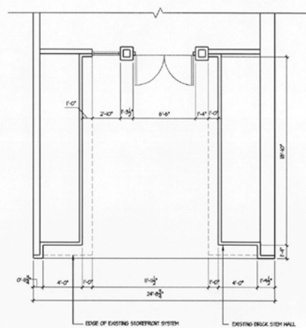
EXISTING ENTRY PLAN SCALE: 1/4" = 1'-0"
