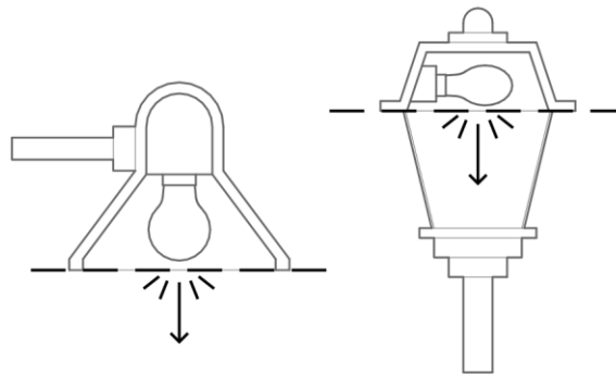
Fig. 20-15-A. Example of Required Light Cutoff
